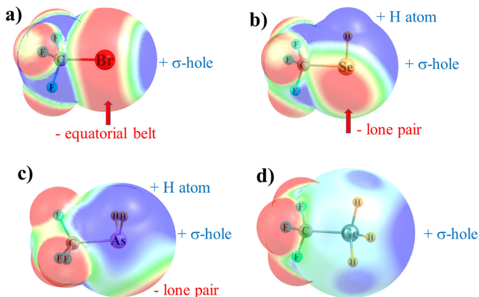
Fig. 6 Molecular electrostatic potentials surrounding a CF 3 Br, b CF 3 SeH, c CF 3 AsH 2 , and d CF 3 GeH 3 . Blue and red regions indicate positive and negative potential, respectively
