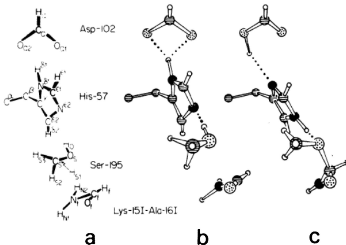
Fig. 1 Identities and dispositions of key catalytic residues in chymotrypsin [6]. Bound state of substrate is shown in part b, including HBs as broken lines. Part c illustrates geometry following proton transfers and formation of tetrahedral intermediate. N atoms are solid, C are striped, and O are speckled
