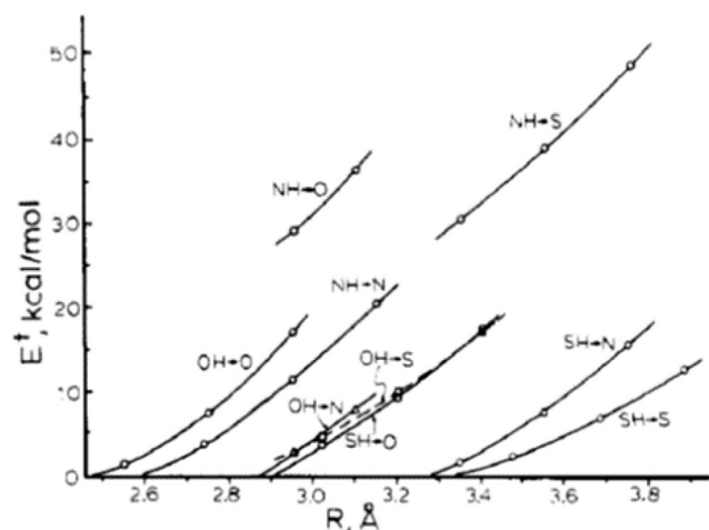
Fig. 3 Proton transfer energy barriers and their relation to H-bond length R [27]. The label on each curve represents the atoms directly involved in the transfer. Systems illustrated are (H_nX-H-YH_m)^+ where H_nX and YH_m = OH_2, NH_3, and SH_2
