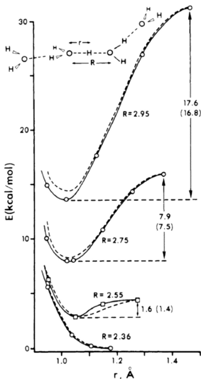
Fig. 2 Left half of proton transfer potentials [10] for (H _5 O _2 ) ^+ (broken curves) and (H _9 O _4 ) ^+ (solid curves). Energy barriers for dimers in parentheses
