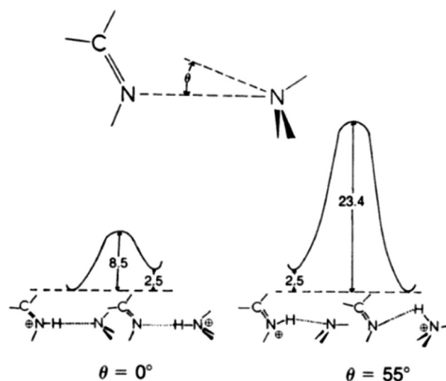
Fig. 4 Proton transfer potentials (kcal/mol) for H_2C=NH and NH_3 . Intermolecular R(N..N) = 2.75 Å and \theta(CN..N) = 129^\circ
